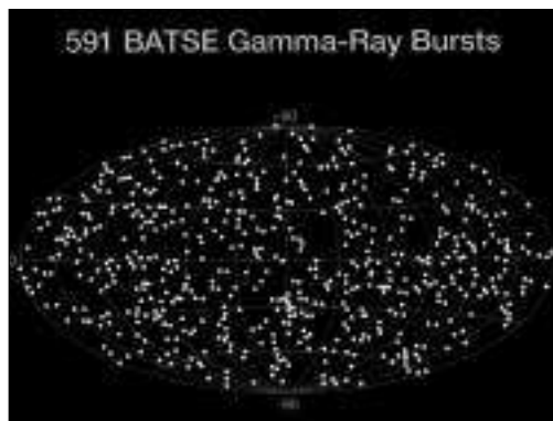
Gamma ray bursts detected by the Compton Gamma Ray Observatory
